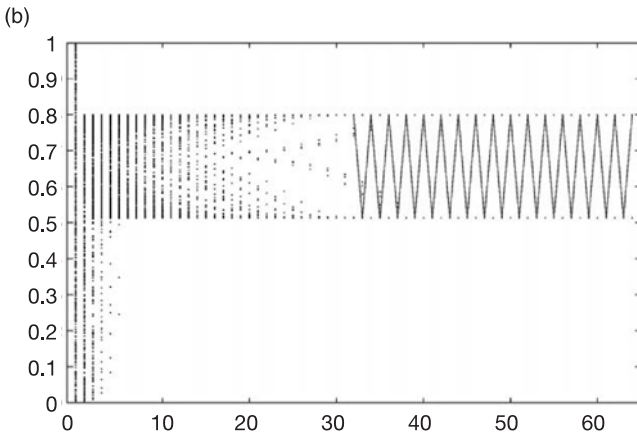
9. Each frame shows the evolution of 512 points, initially spread at random between zero and one, as they move forward under the Logistic Map. Each panel shows one of four different values of a , showing the collapse towards (a) a fixed point, (b) a period two loop, (c) a period four loop, and (d) chaos. The solid line starting at time 32 shows the trajectory of one point, in order to make the path on each attractor visible
